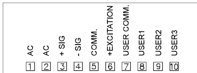
Anschlüsse PAXS0000
